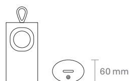
Lunari 83 x 60 x 160 mm [L x B/W x H]
