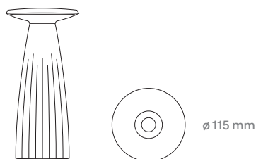
Nuflair Rechargeable Table Lamp 85 x 240 mm [W x H]
